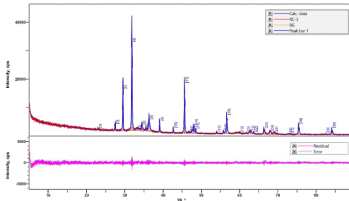
Figure. 09. XRD analysis of ZnO Nps
