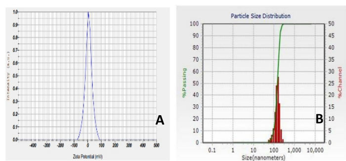
Figure 10. A) Zeta potential and B) DLS analysis of ZnO Nps.
