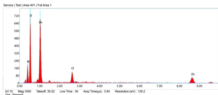
Figure. 08. EDX analysis of ZnO Nps
