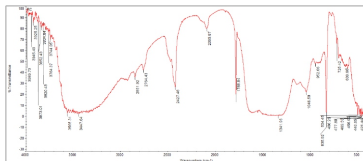
Figure. 06. FTIR analysis of H. lobatus ZnO Nps
